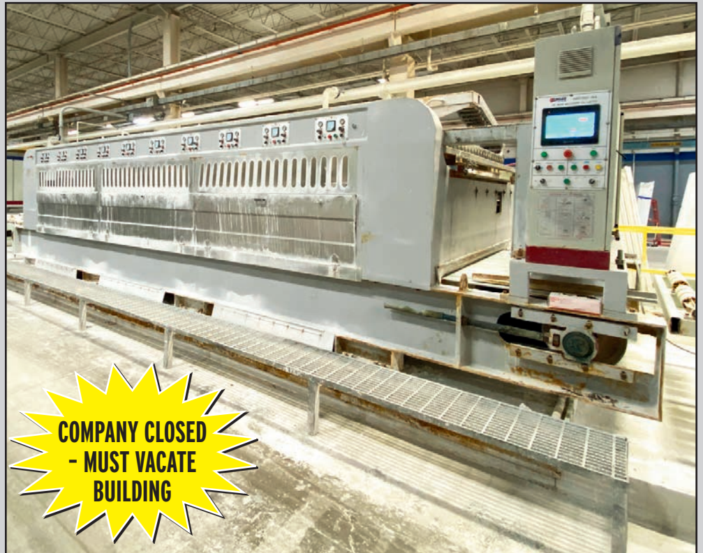
(1 OF 2) 16-HEAD CNC POLISHING MACHINES
